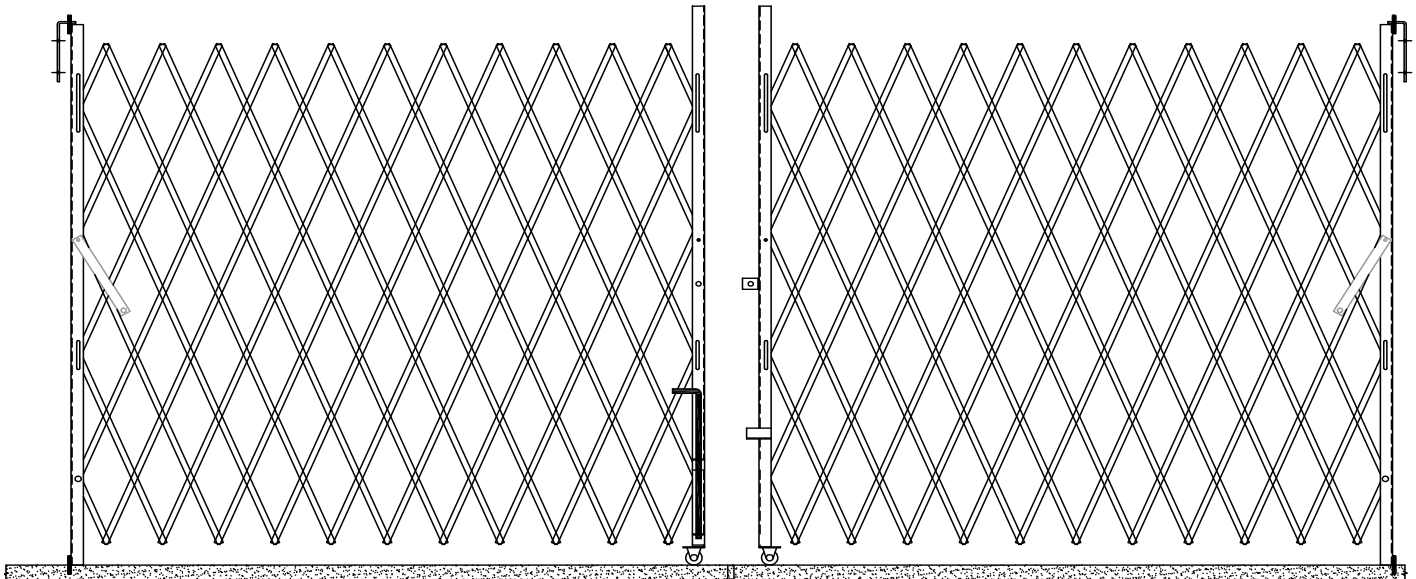
Double gates for openings up to 16' (4,877 mm) wide.
